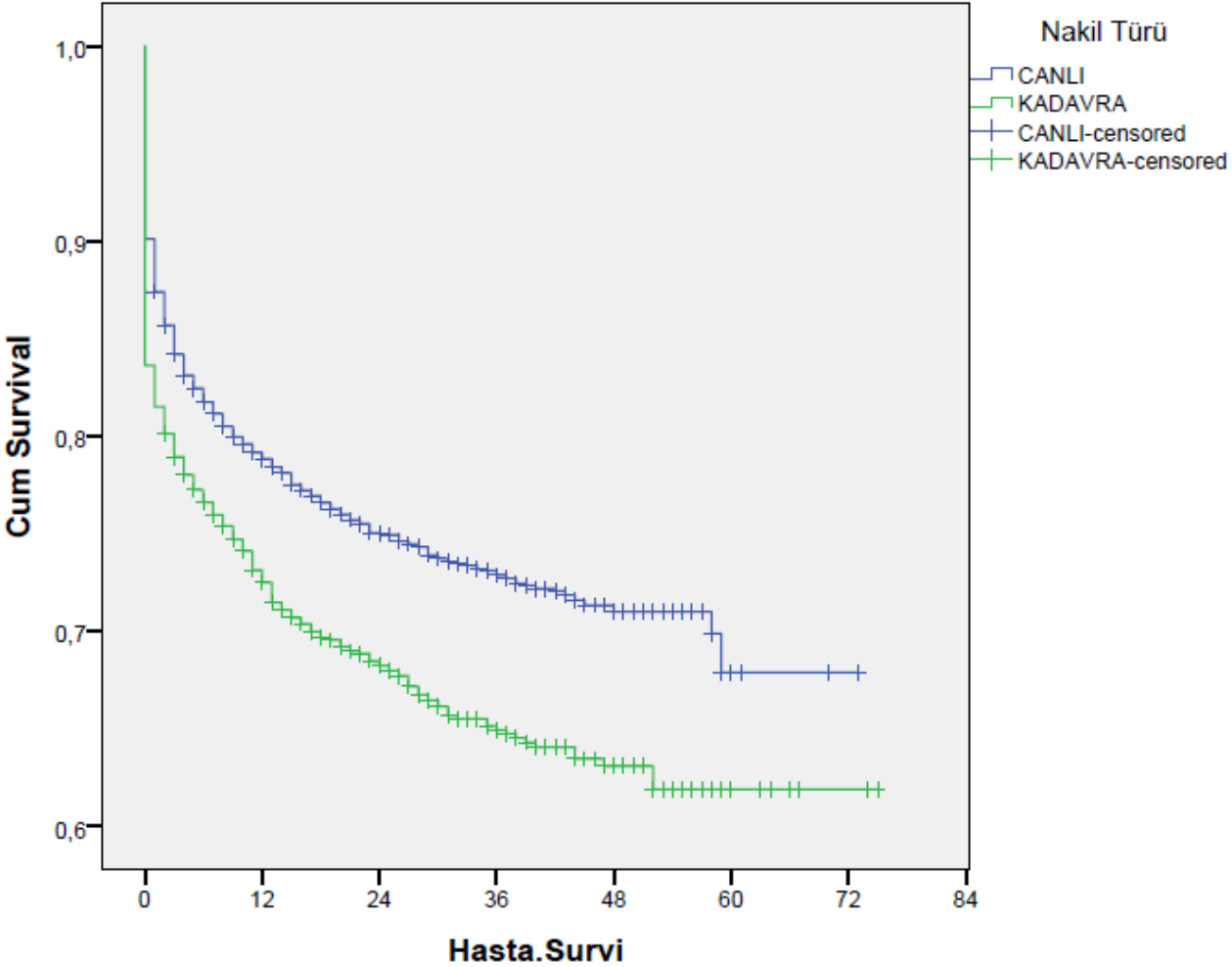
Survival Functions
